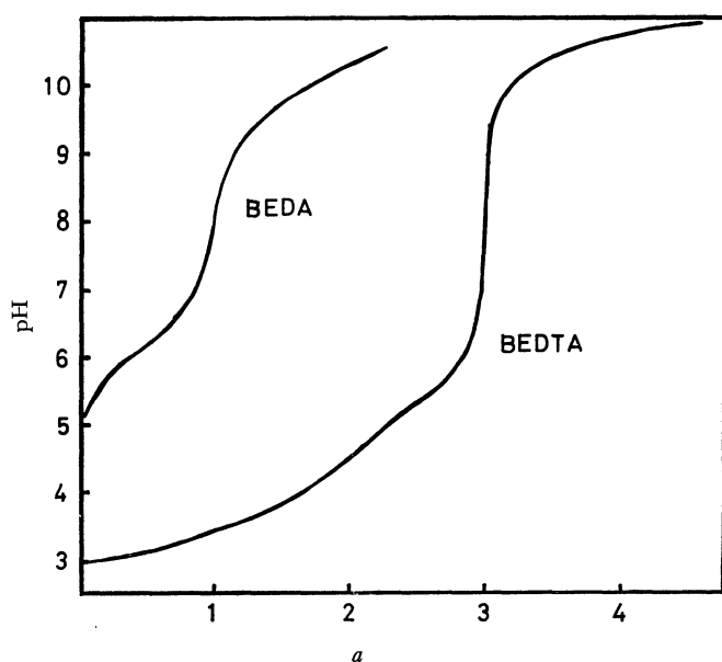
Fig. 1. The pH titration curves of BEDA and BEDTA at 25^\circ\text{C} in 0.1 M KCl.
